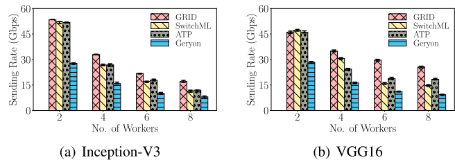
Fig. 5. Gradient sending rate vs. no. of workers.
