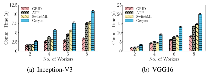
Fig. 6. Communication time vs. no. of workers.
